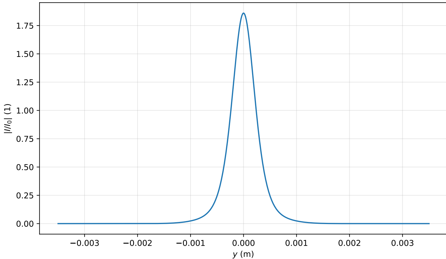
Intensity profile I(x=0, y, z=1.513)/I_0 , P_{in}=1.0P_{cr} , artificial time
